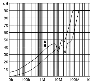
32 A types
