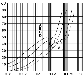
100 A types
