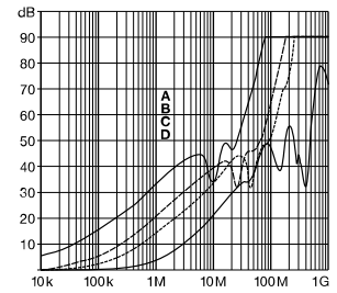
63 A types
