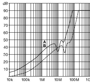
16 A types
