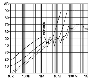
200 A types
