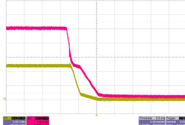
Shutdown Input: 5.0V
