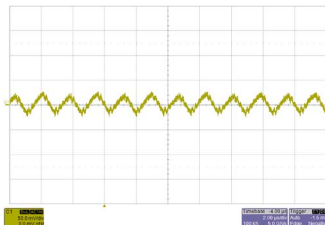
Ripple and Noise (0~20MHz) Input: 3.6V, Output: 5V, Load: 1A
