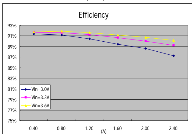
Efficiency
