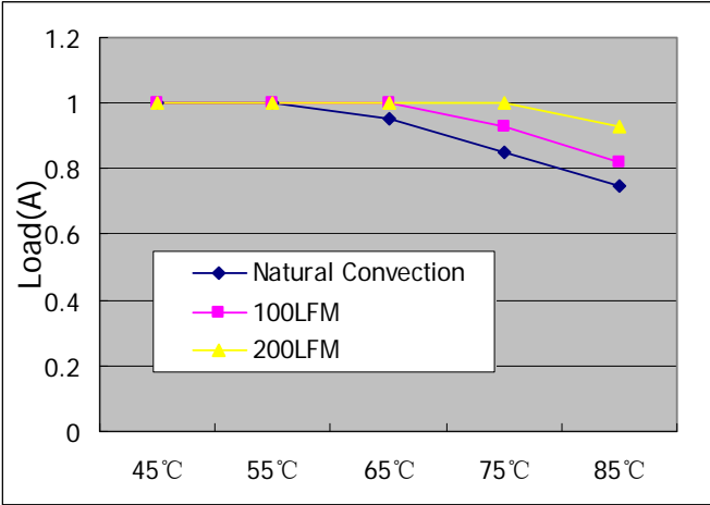
Derating Curve (Vin=3.3V)
