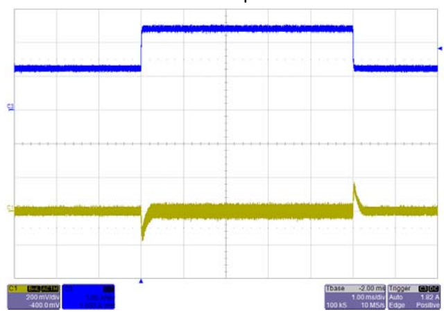
Transient Response (C1: output, C3: Load Current) Load current Step from 1A~2A~1A, 0.1A/uS Input: 3.6V
