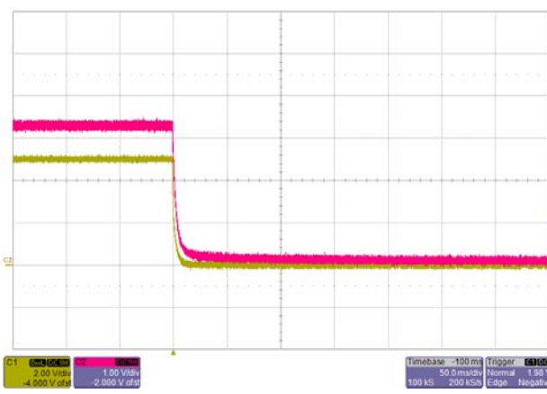
Shutdown Input:3.6V
