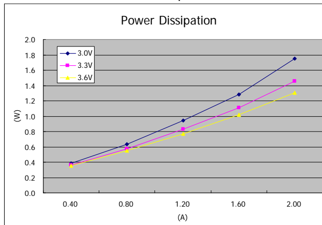
Power Dissipation
