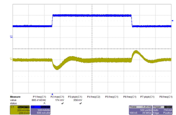
Transient Response (C1: output, C3: Load Current) Load current Step from 0.5A~1A~0.5A, 0.1A/uS Input: 5.0V, Output: 12V
