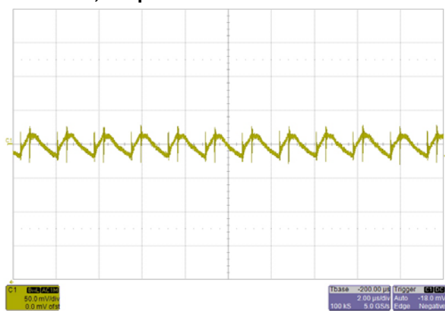
Ripple and Noise (0~20MHz) Input: 3.3V, Output: 5V, Load: 1A
