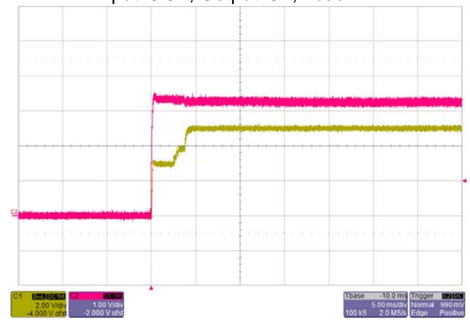
Start-up Input:3.3V
