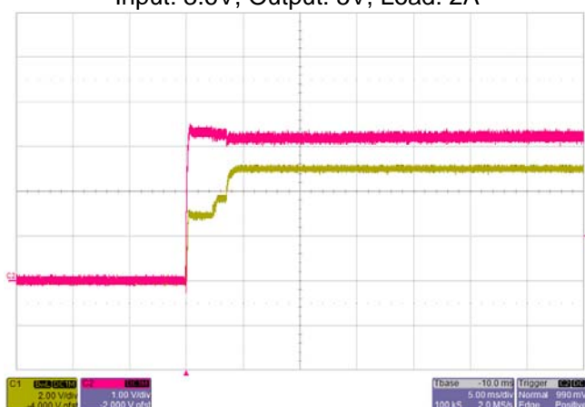
Start-up Input:3.6V
