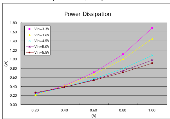
Power Dissipation
