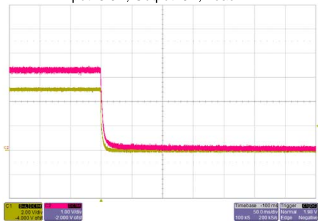
Shutdown Input:3.3V
