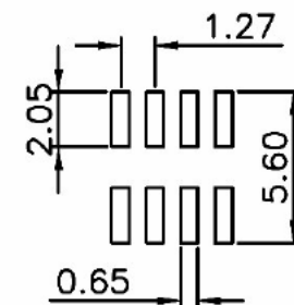
Recommended P.C.B Layout (Tolerance: ±0.05)
