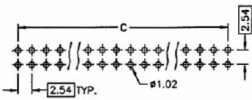
RECOMMEND P.C.B. LAYOUT BOTTOM VIEW
