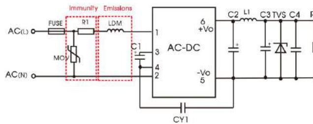
Recommended circuit 4
