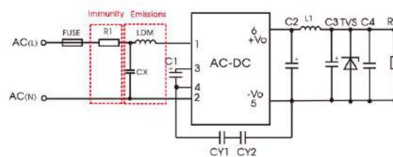
Recommended circuit 2
