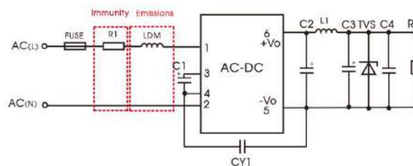
recommended circuit 1
