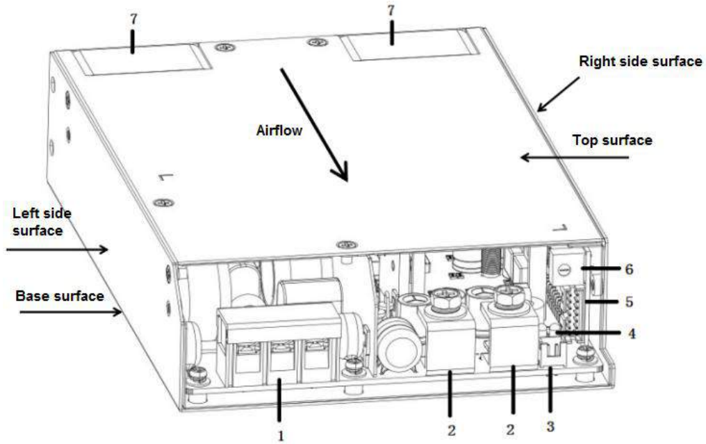
Fig. 1: Appearance information of SLMF1000-20Bxx
