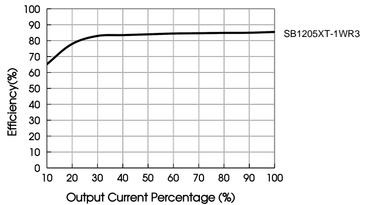
Efficiency Vs Output Load (Vin=12V)
