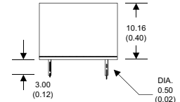
16 Pin DIL Package Non-Conductive Plastic
