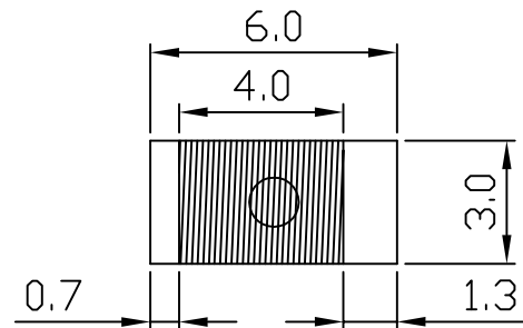
SOLDER PAD Dimension
